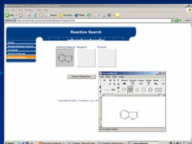
Reaction prediction and in silico piloting
